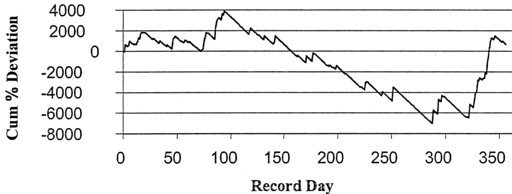
Figure 5.2: Cumulative percent deviation relative to the average of fog water (zero line) collected at Klipneus. The graph increases whenever the fog water exceeds the mean and decreases when it is below the mean. Long periods without fog cause a decline.
