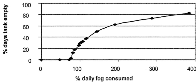
Figure 5.4: Number of days per year that the tank is empty depending on the rate of water consumption relative to the average daily supply.
