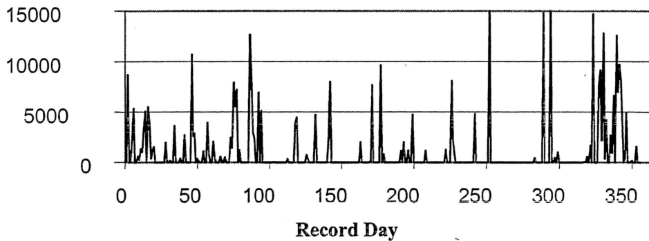
Figure 5.1: Daily records of fog water collected at Klipneus.
