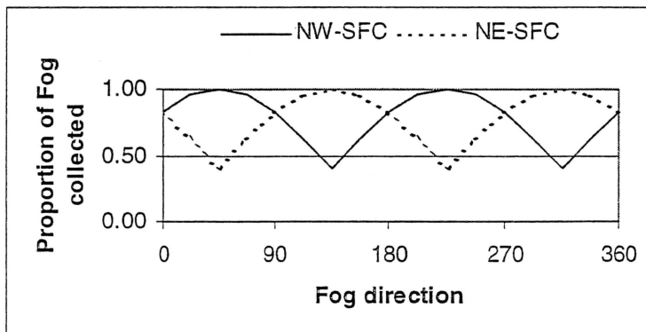
Figure A3.1: Proportion of fog from various directions collected by two SFCs oriented NW and NE.
