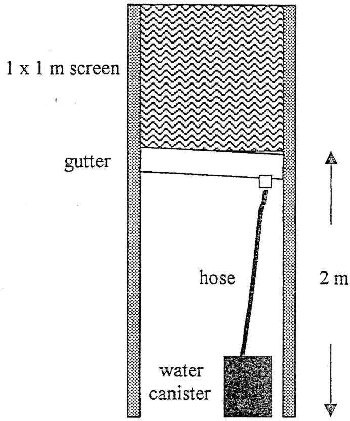
Figure A2.1: Illustration of a Standard Fog Collector.
